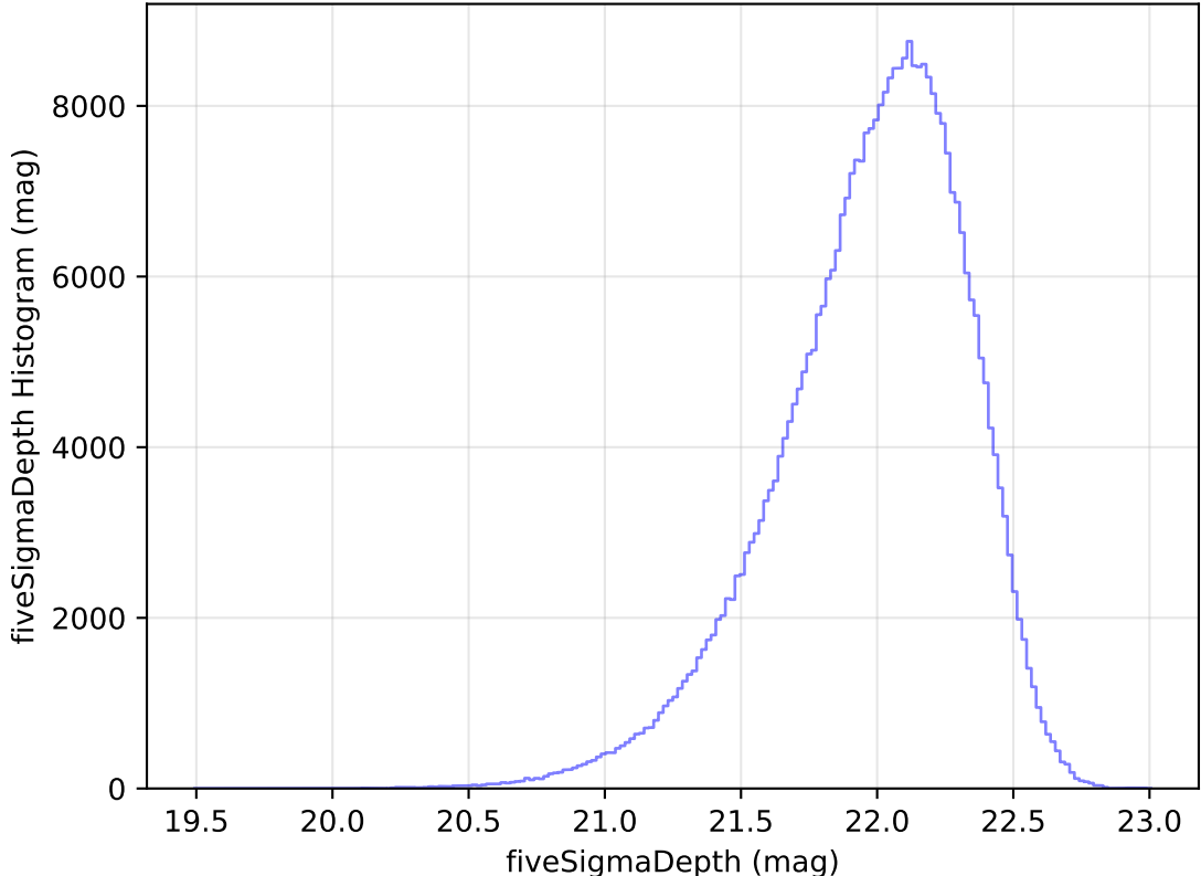
too_elab_heavy_r32_d2_gz_v3.4_10yrs All sky y band: fiveSigmaDepth Histogram
