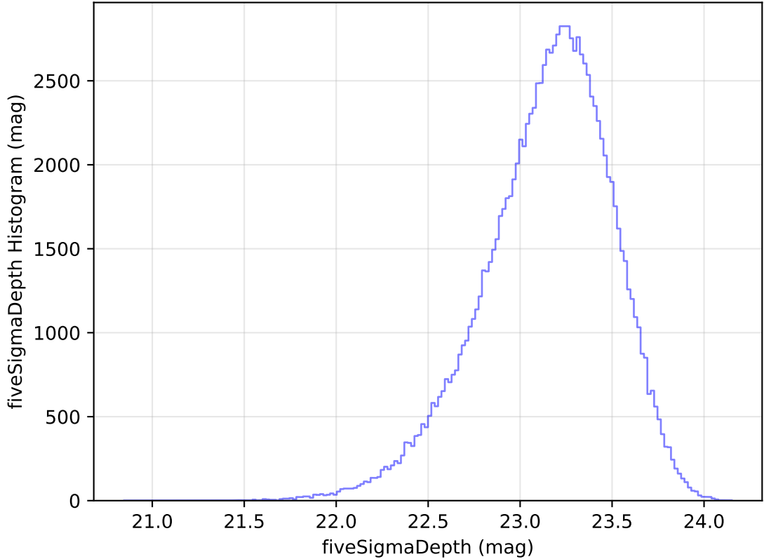
too_elab_heavy_r32_d2_gz_v3.4_10yrs All sky u band: fiveSigmaDepth Histogram
