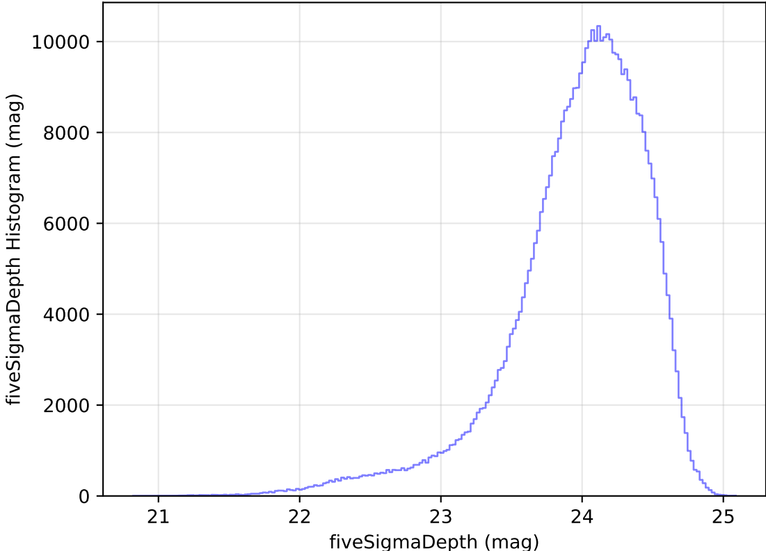
too_elab_heavy_r32_d2_gz_v3.4_10yrs All sky r band: fiveSigmaDepth Histogram
