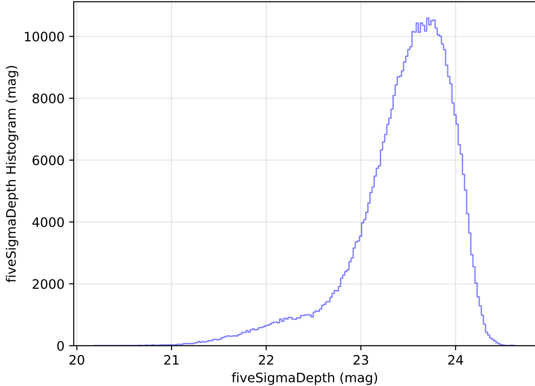
too_elab_heavy_r32_d2_gz_v3.4_10yrs All sky i band: fiveSigmaDepth Histogram
