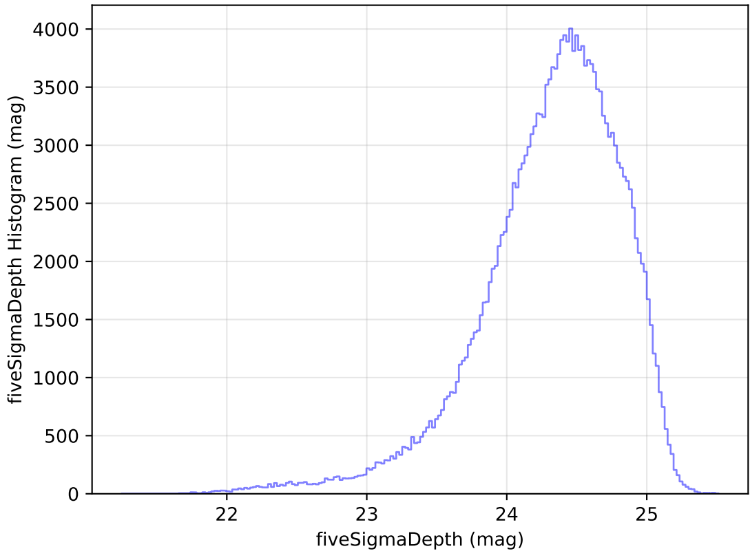
too_elab_heavy_r32_d2_gz_v3.4_10yrs All sky g band: fiveSigmaDepth Histogram
