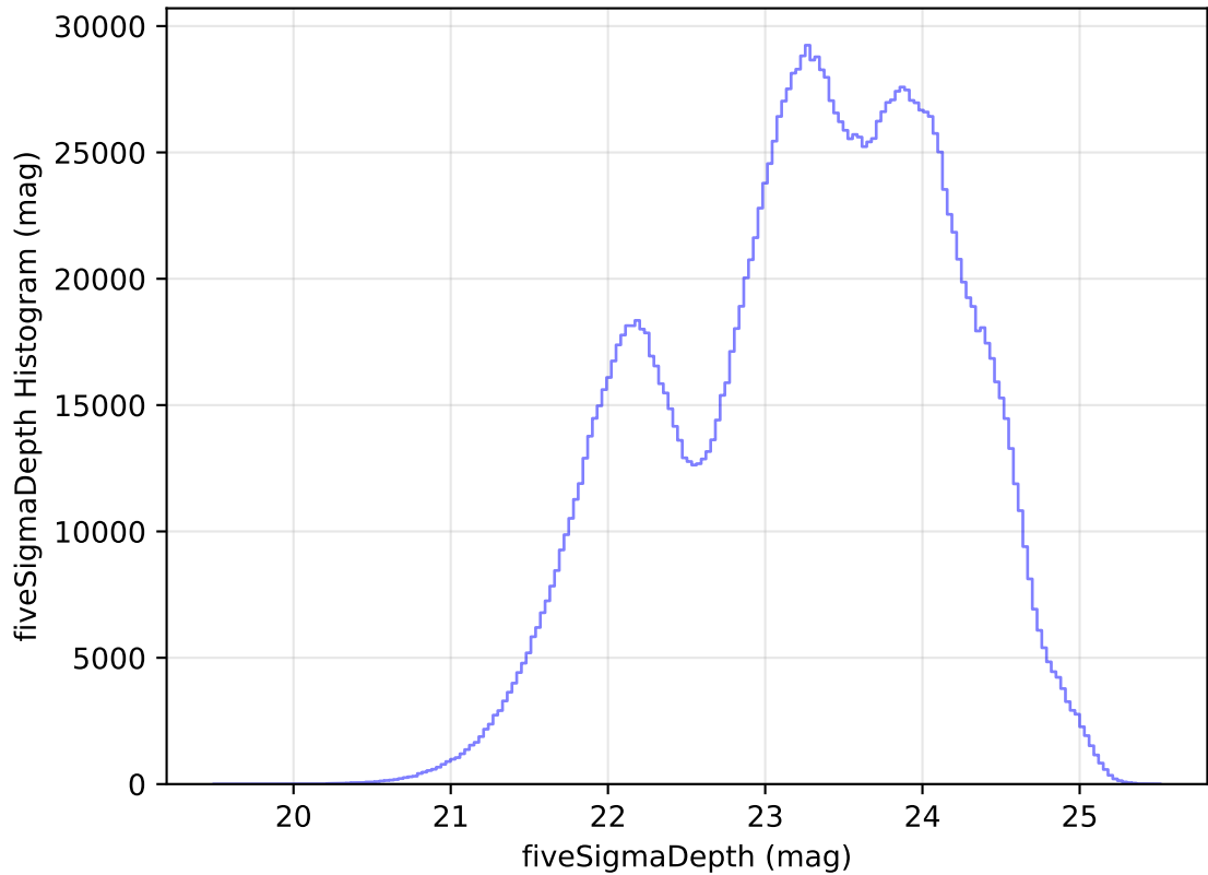
too_elab_heavy_r32_d2_gz_v3.4_10yrs All sky all bands: fiveSigmaDepth Histogram
