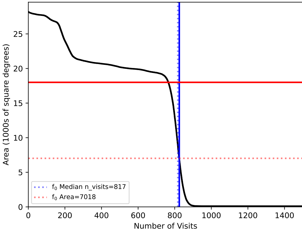
too_elab_heavy_r32_d2_gz_v3.4_10yrs All sky: f0
