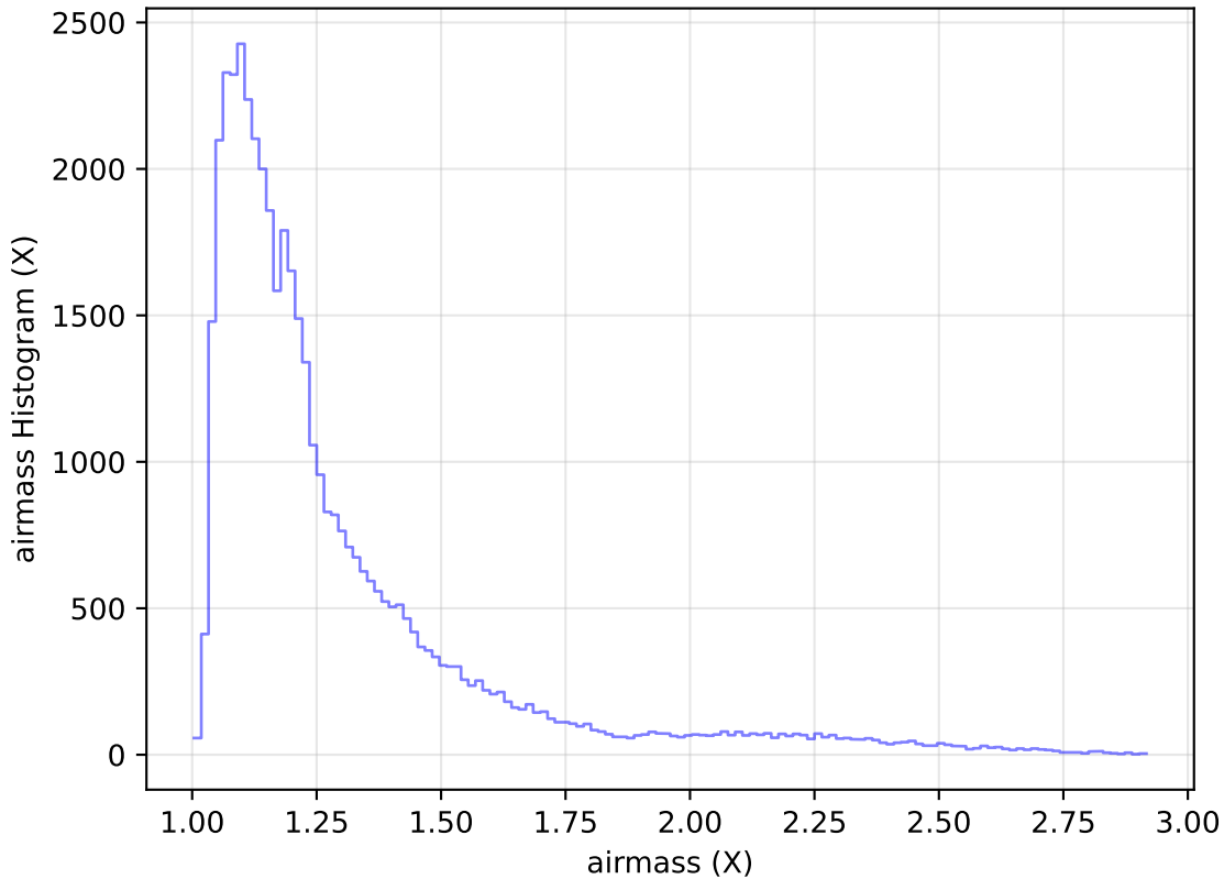
too_elab_heavy_r32_d2_gz_v3.4_10yrs Yr 1 z band: airmass Histogram
