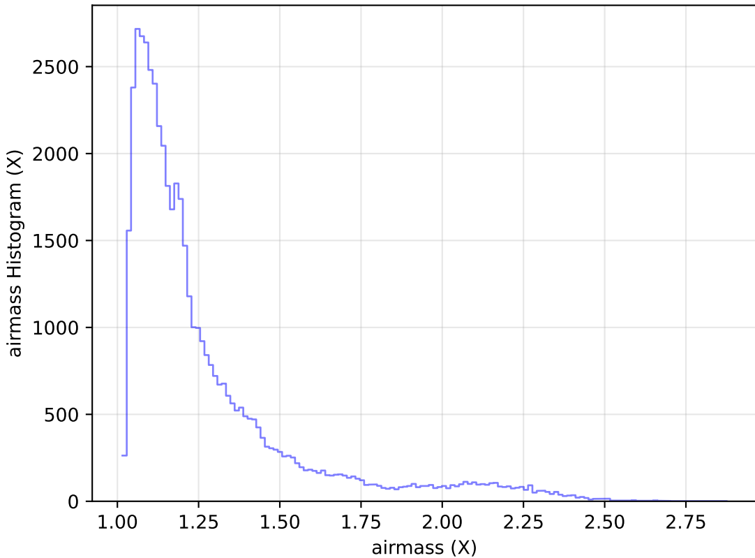
too_elab_heavy_r32_d2_gz_v3.4_10yrs Yr 1 r band: airmass Histogram
