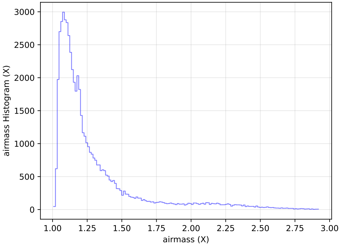
too_elab_heavy_r32_d2_gz_v3.4_10yrs Yr 1 i band: airmass Histogram
