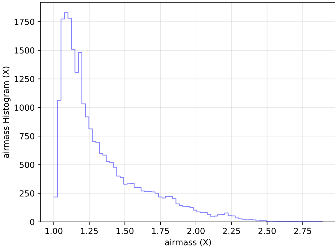
too_elab_heavy_r32_d2_gz_v3.4_10yrs Yr 1 g band: airmass Histogram
