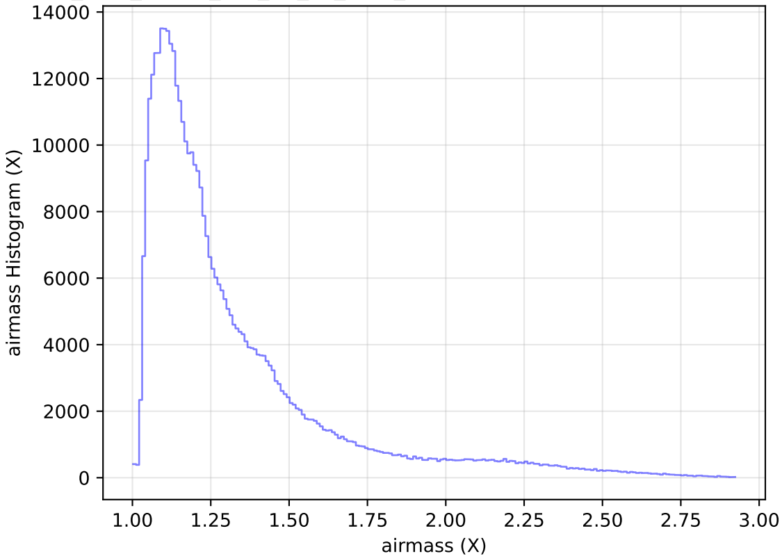
too_elab_heavy_r32_d2_gz_v3.4_10yrs WFD z band: airmass Histogram
