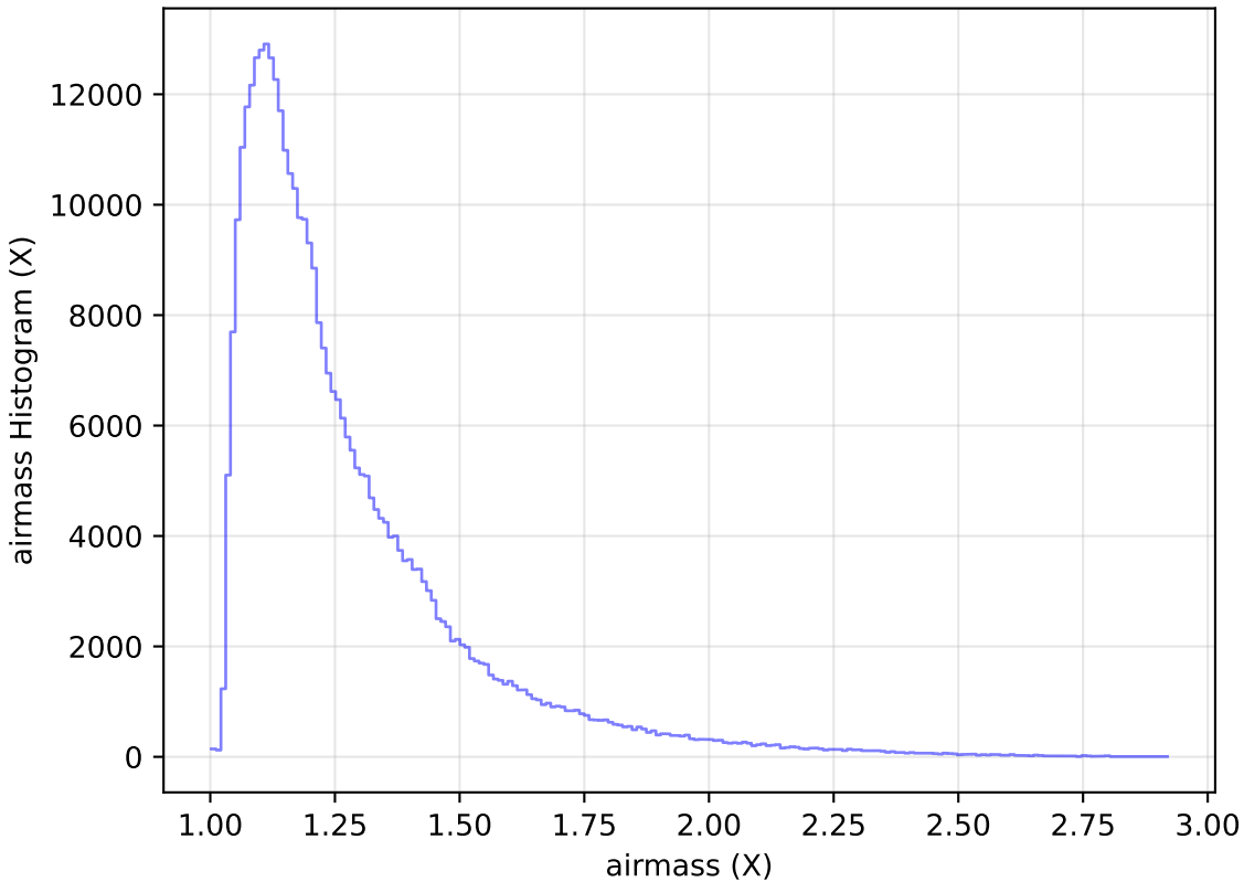
too_elab_heavy_r32_d2_gz_v3.4_10yrs WFD y band: airmass Histogram
