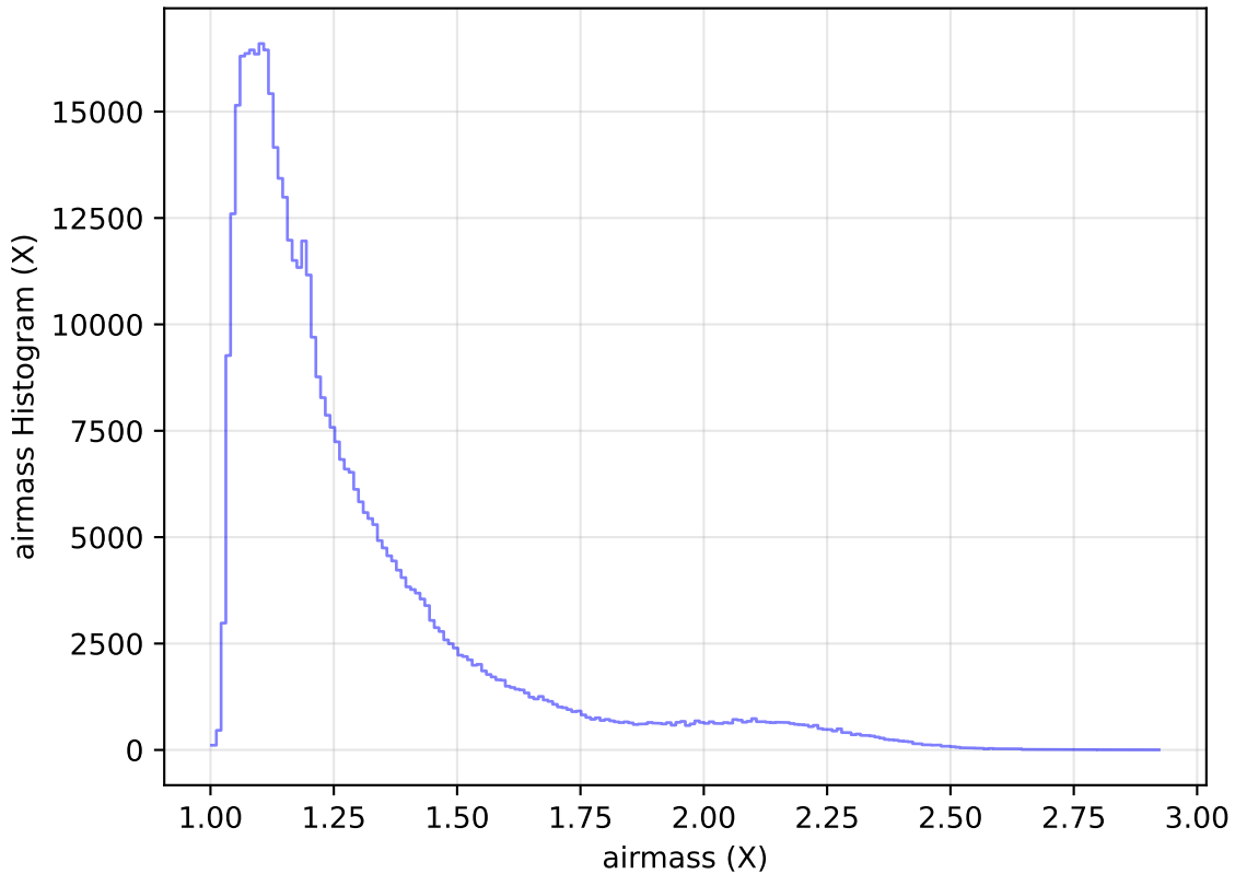
too_elab_heavy_r32_d2_gz_v3.4_10yrs WFD r band: airmass Histogram
