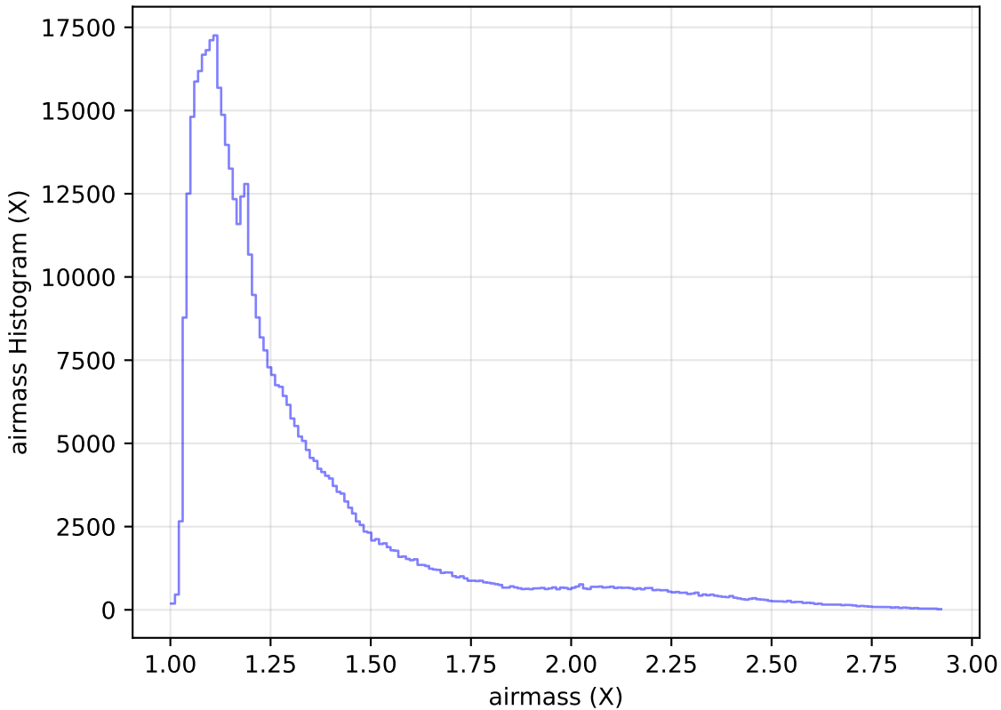
too_elab_heavy_r32_d2_gz_v3.4_10yrs WFD i band: airmass Histogram
