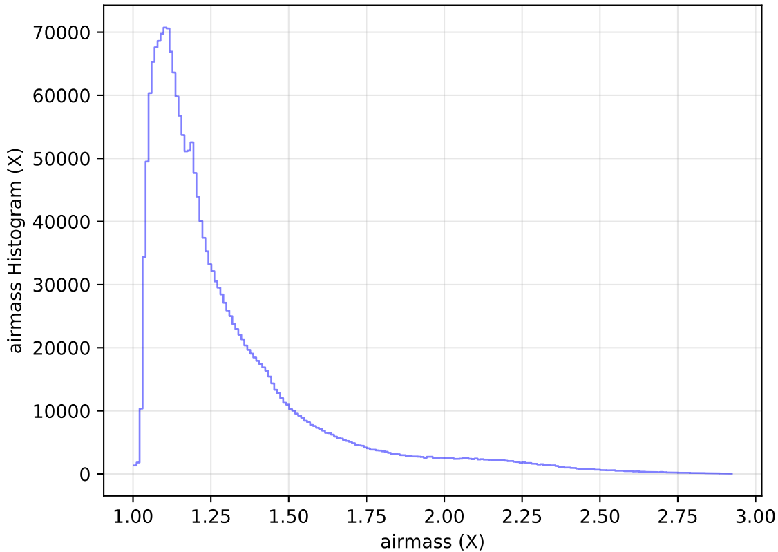
too_elab_heavy_r32_d2_gz_v3.4_10yrs WFD all bands: airmass Histogram
