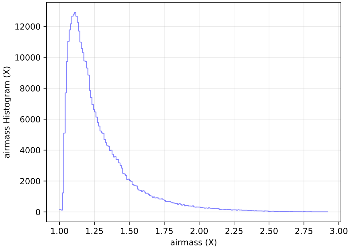
too_elab_heavy_r32_d2_gz_v3.4_10yrs All sky y band: airmass Histogram
