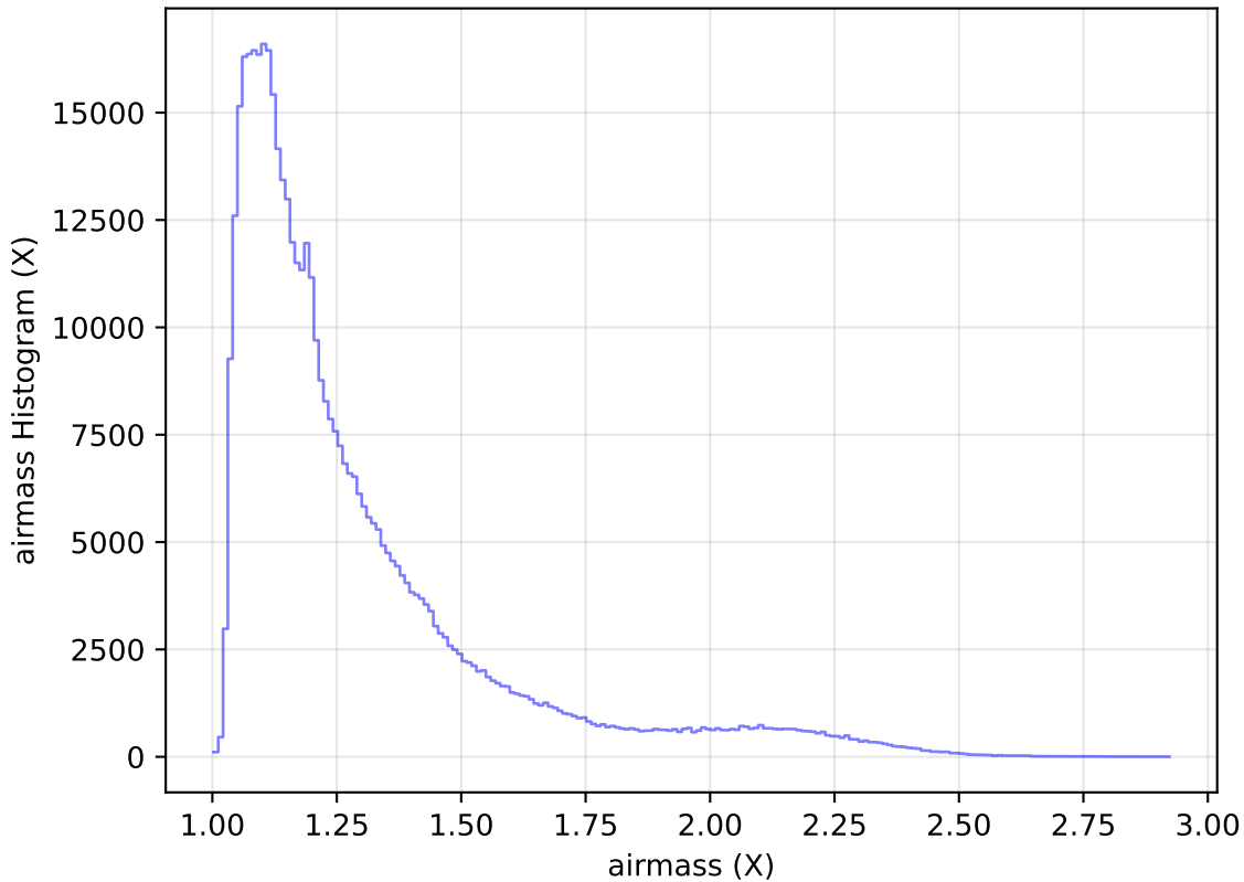
too_elab_heavy_r32_d2_gz_v3.4_10yrs All sky r band: airmass Histogram
