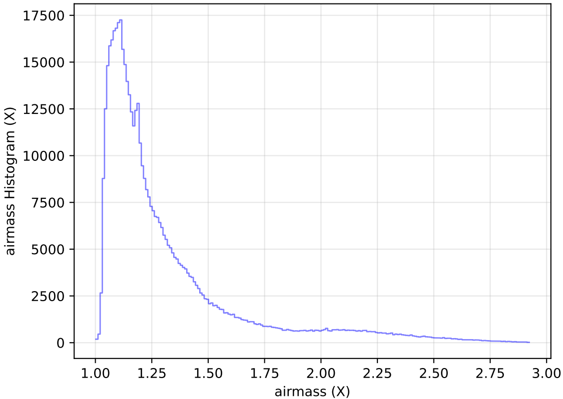
too_elab_heavy_r32_d2_gz_v3.4_10yrs All sky i band: airmass Histogram
