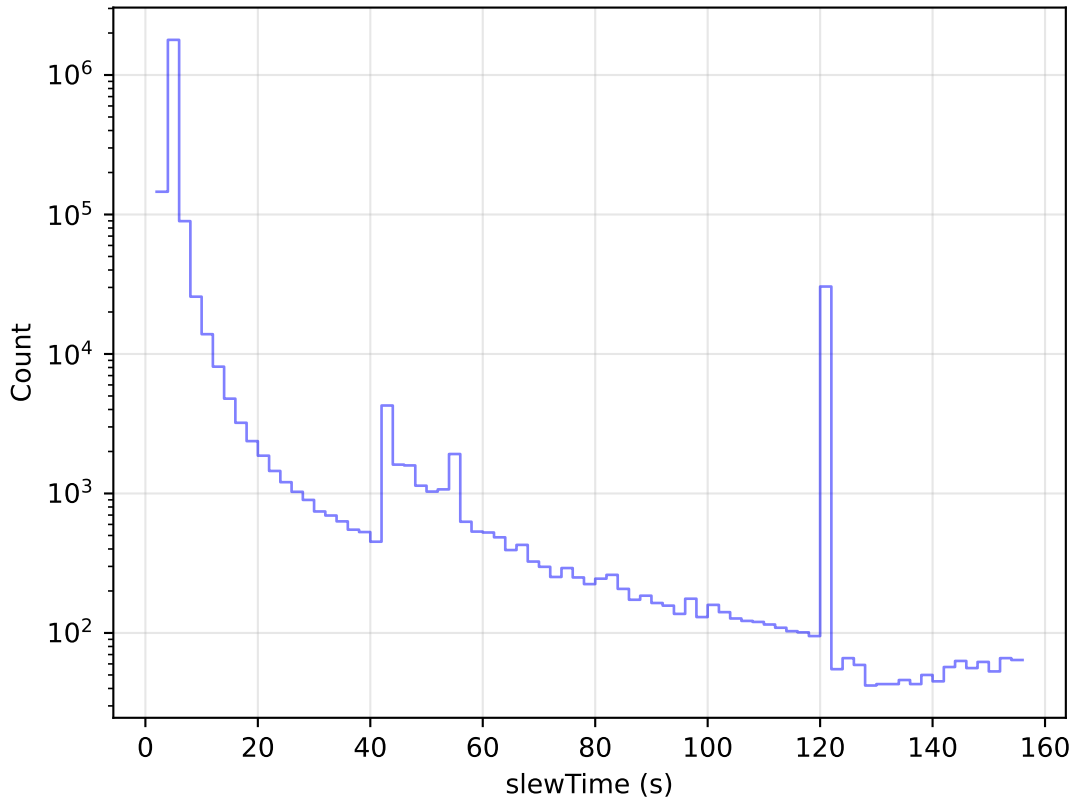
too_elab_heavy_r32_d2_gz_v3.4_10yrs All visits: Slew Time Histogram
