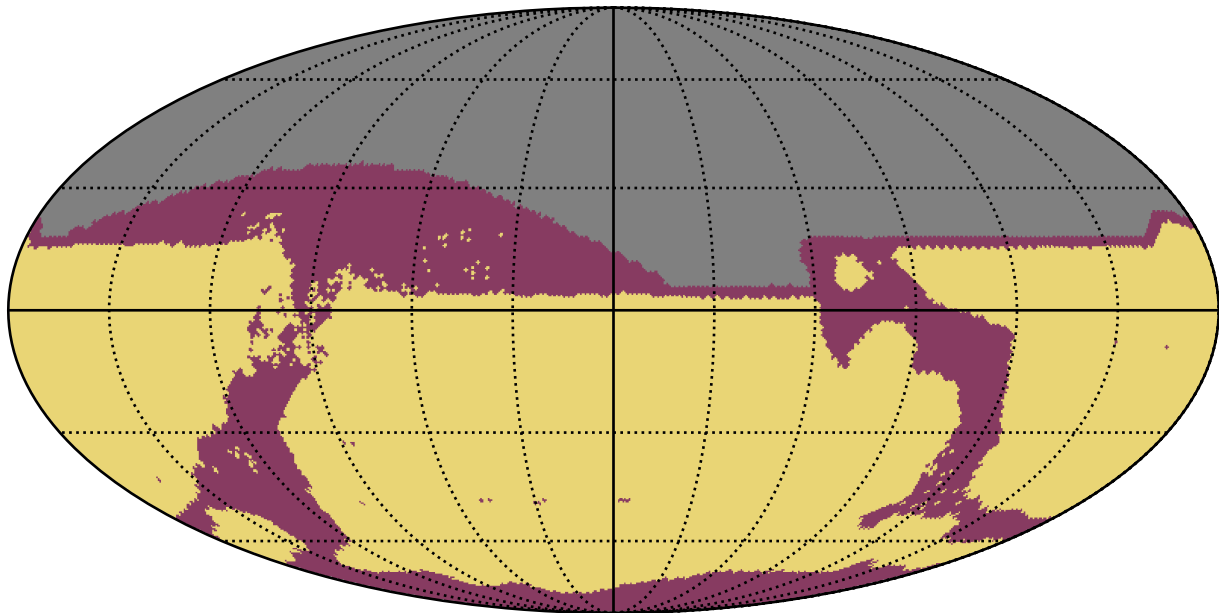
too_elab_heavy_r32_d2_gz_v3.4_10yrs All sky: RapidRevisits
