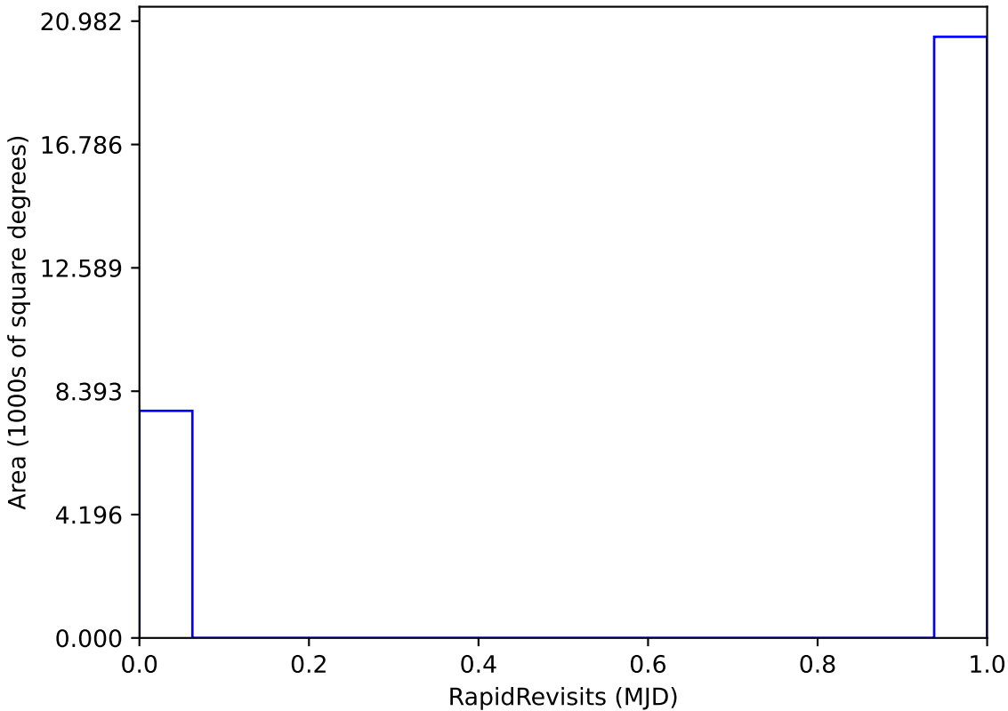
too_elab_heavy_r32_d2_gz_v3.4_10yrs All sky: RapidRevisits
