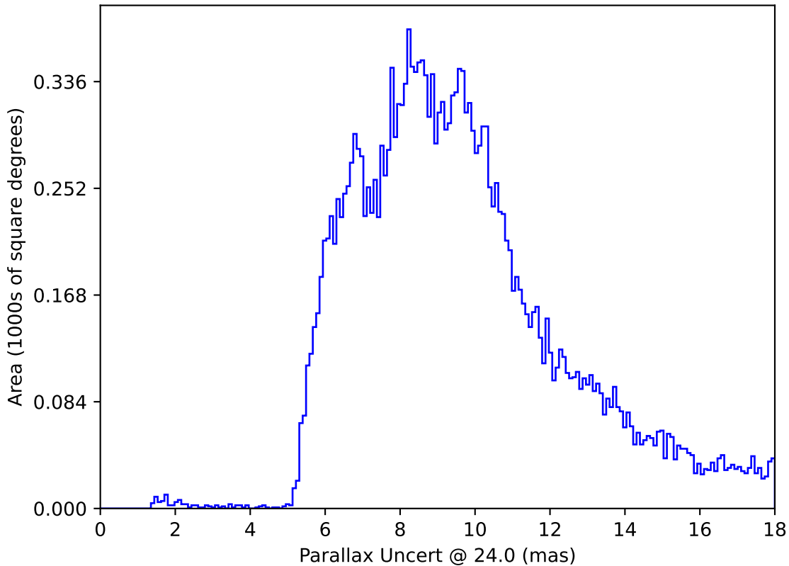
too_elab_heavy_r32_d2_gz_v3.4_10yrs All sky: Parallax Uncert @ 24.0
