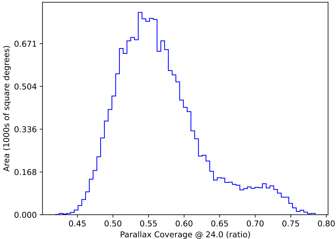
too_elab_heavy_r32_d2_gz_v3.4_10yrs WFD: Parallax Coverage @ 24.0
