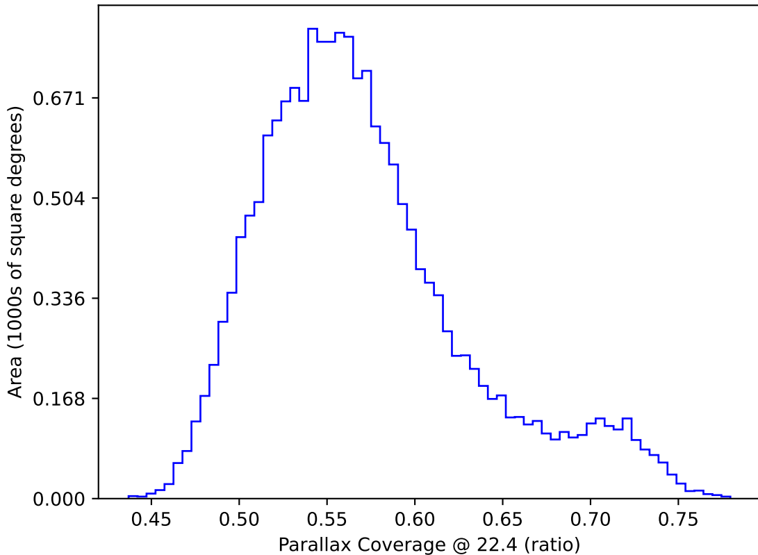
too_elab_heavy_r32_d2_gz_v3.4_10yrs WFD: Parallax Coverage @ 22.4
