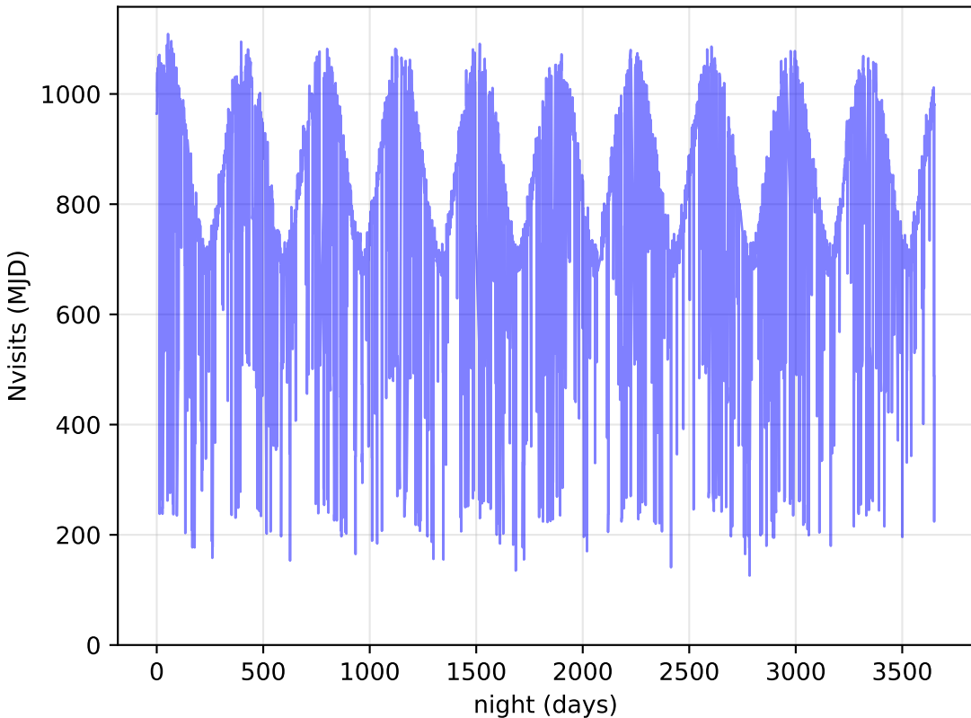
too_elab_heavy_r32_d2_gz_v3.4_10yrs All visits: Nvisits
