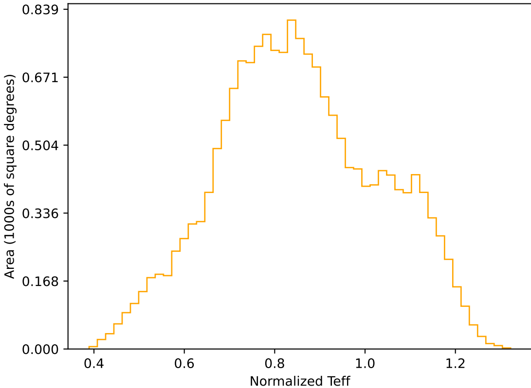
too_elab_heavy_r32_d2_gz_v3.4_10yrs WFD r band: Normalized Teff
