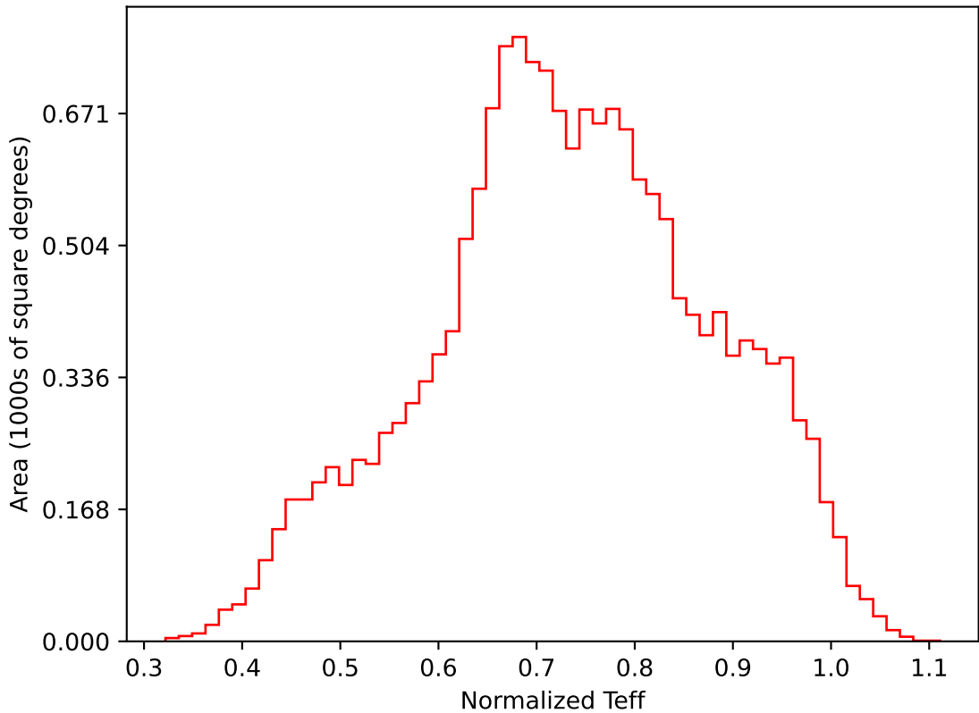
too_elab_heavy_r32_d2_gz_v3.4_10yrs WFD i band: Normalized Teff
