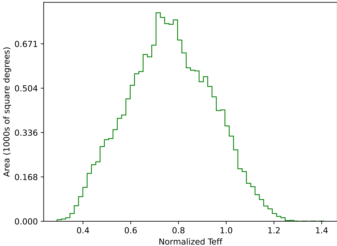
too_elab_heavy_r32_d2_gz_v3.4_10yrs WFD g band: Normalized Teff
