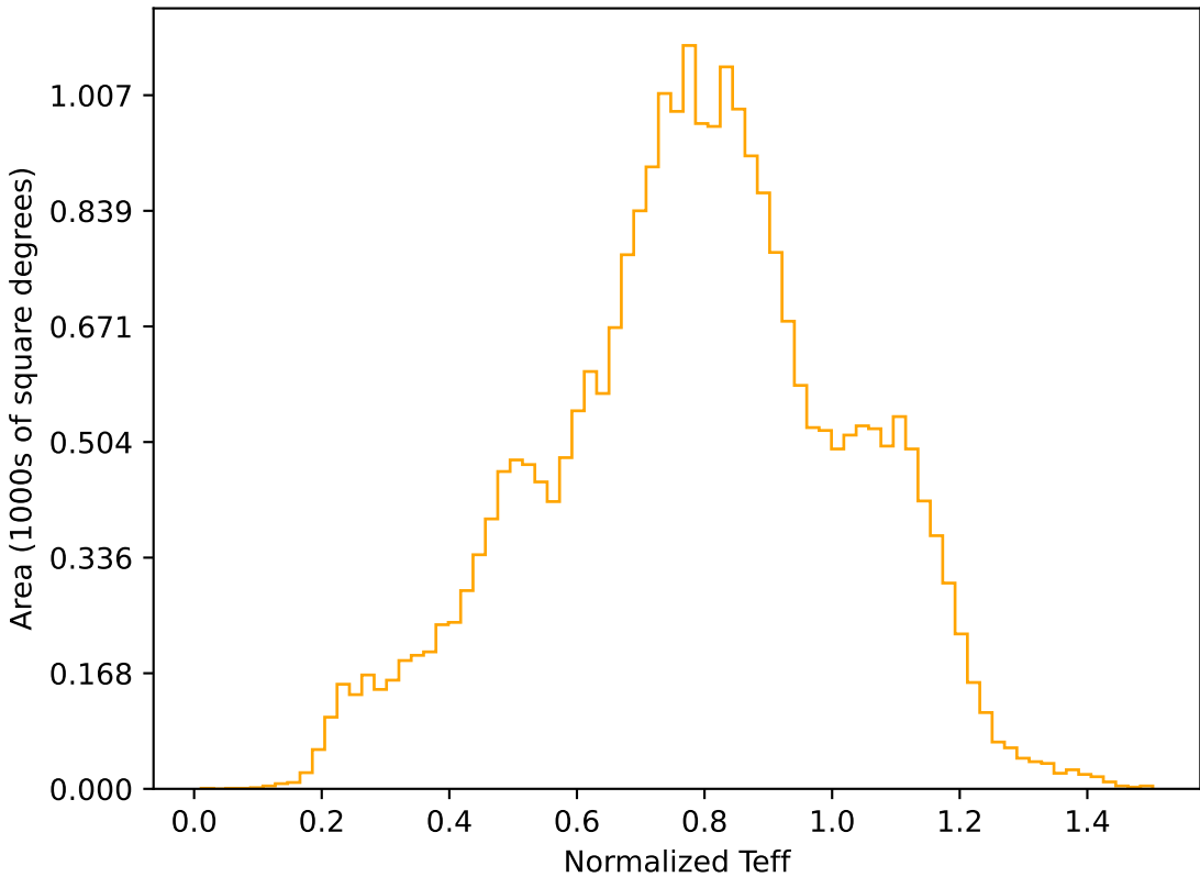
too_elab_heavy_r32_d2_gz_v3.4_10yrs All sky r band: Normalized Teff
