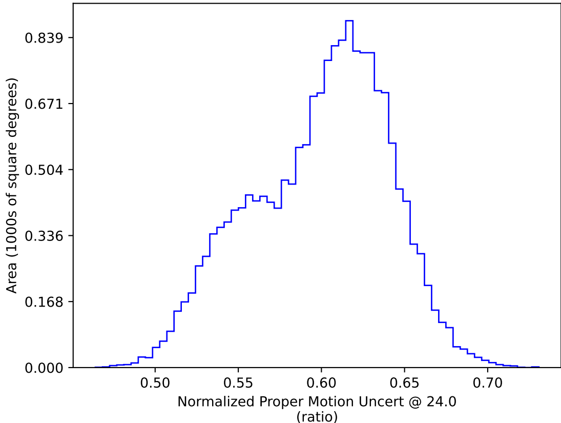
too_elab_heavy_r32_d2_gz_v3.4_10yrs WFD: Normalized Proper Motion Uncert @ 24.0
