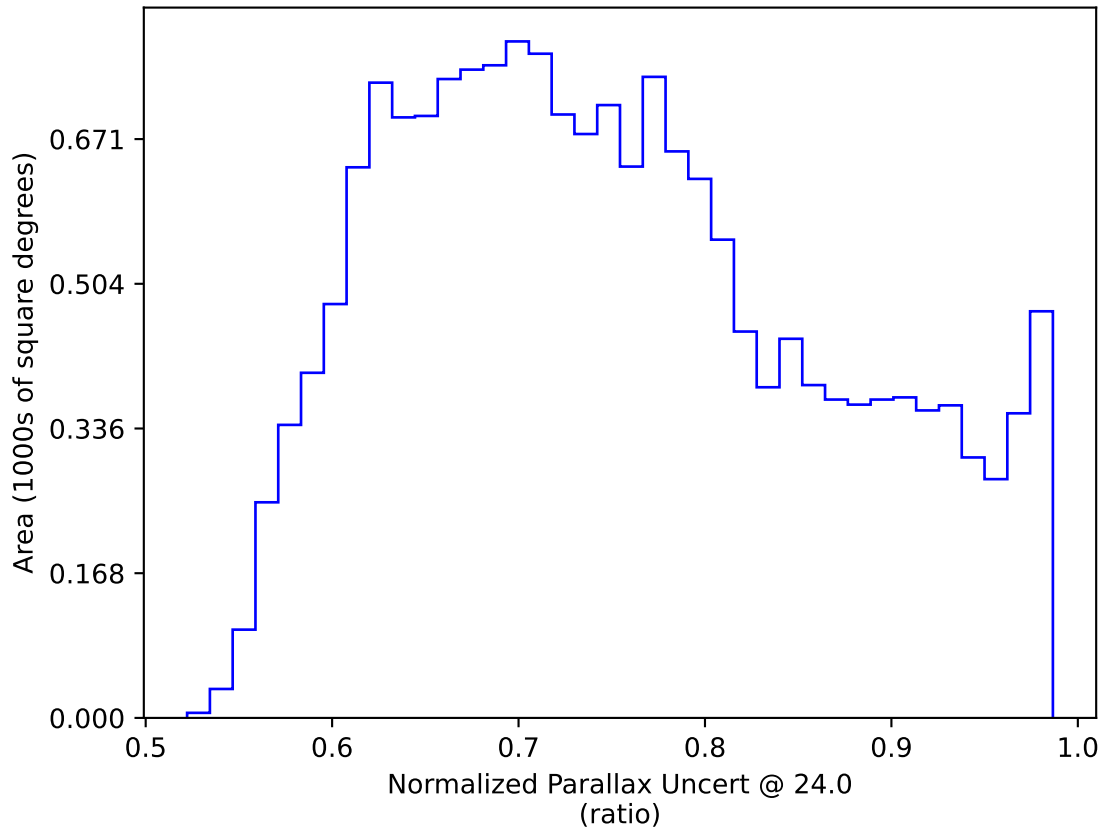
too_elab_heavy_r32_d2_gz_v3.4_10yrs WFD: Normalized Parallax Uncert @ 24.0
