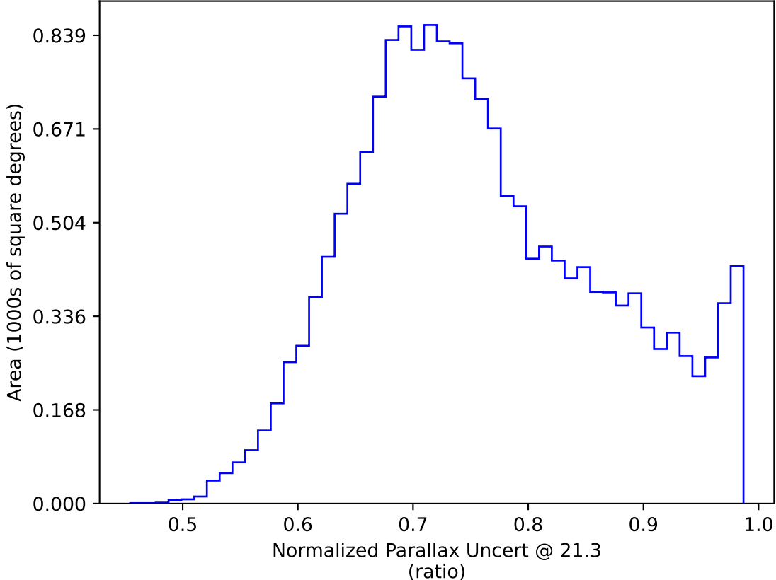
too_elab_heavy_r32_d2_gz_v3.4_10yrs WFD y band only: Normalized Parallax Uncert @ 21.3
