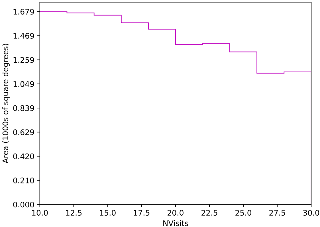
too_elab_heavy_r32_d2_gz_v3.4_10yrs Yr 3-4 z band: NVisits
