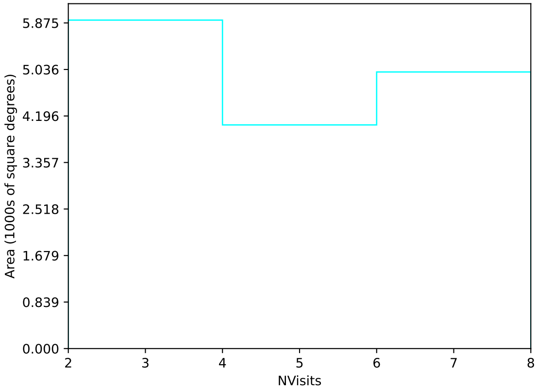
too_elab_heavy_r32_d2_gz_v3.4_10yrs Yr 3-4 u band: NVisits
