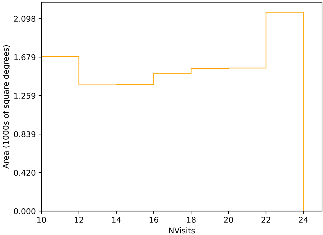
too_elab_heavy_r32_d2_gz_v3.4_10yrs Yr 3-4 r band: NVisits
