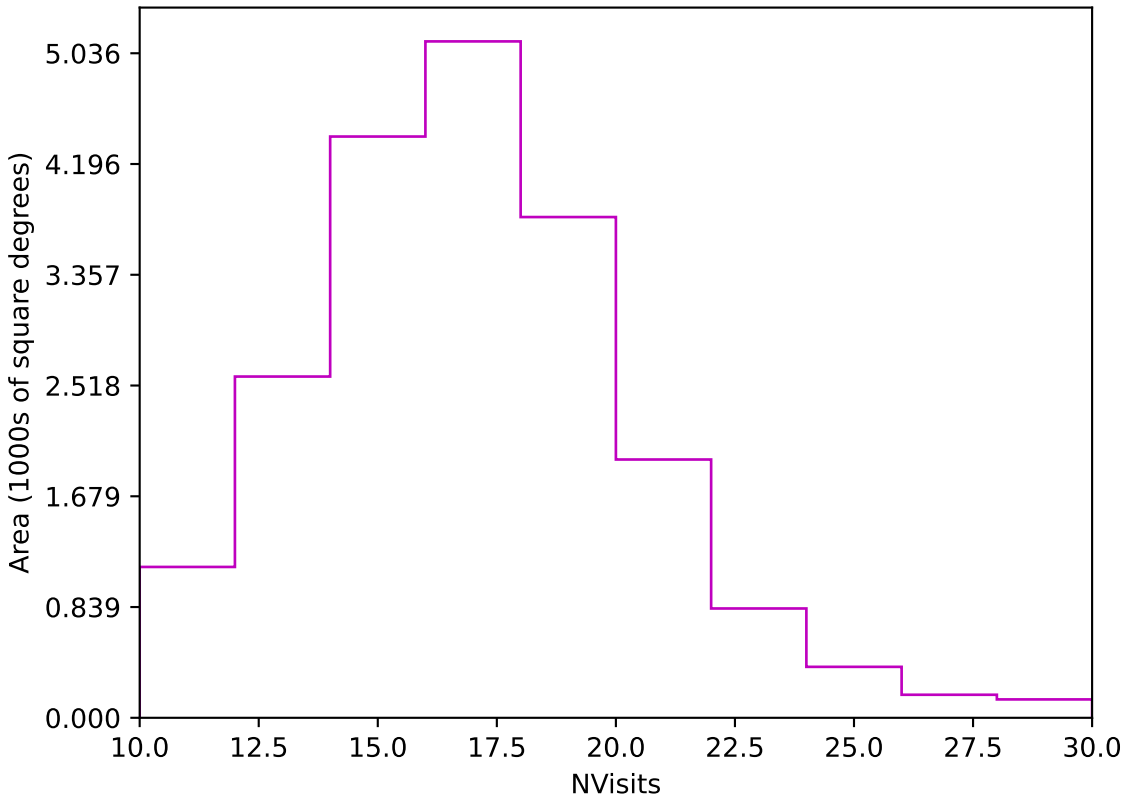
too_elab_heavy_r32_d2_gz_v3.4_10yrs Yr 1 z band: NVisits
