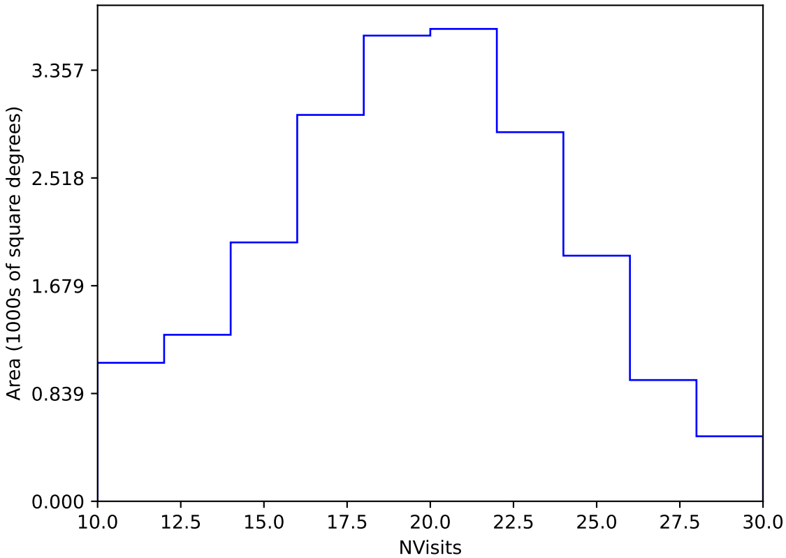
too_elab_heavy_r32_d2_gz_v3.4_10yrs Yr 1 y band: NVisits
