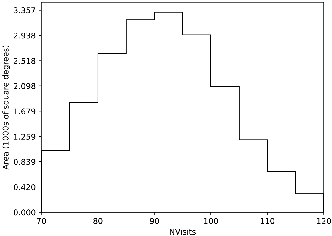
too_elab_heavy_r32_d2_gz_v3.4_10yrs Yr 1 all bands: NVisits
