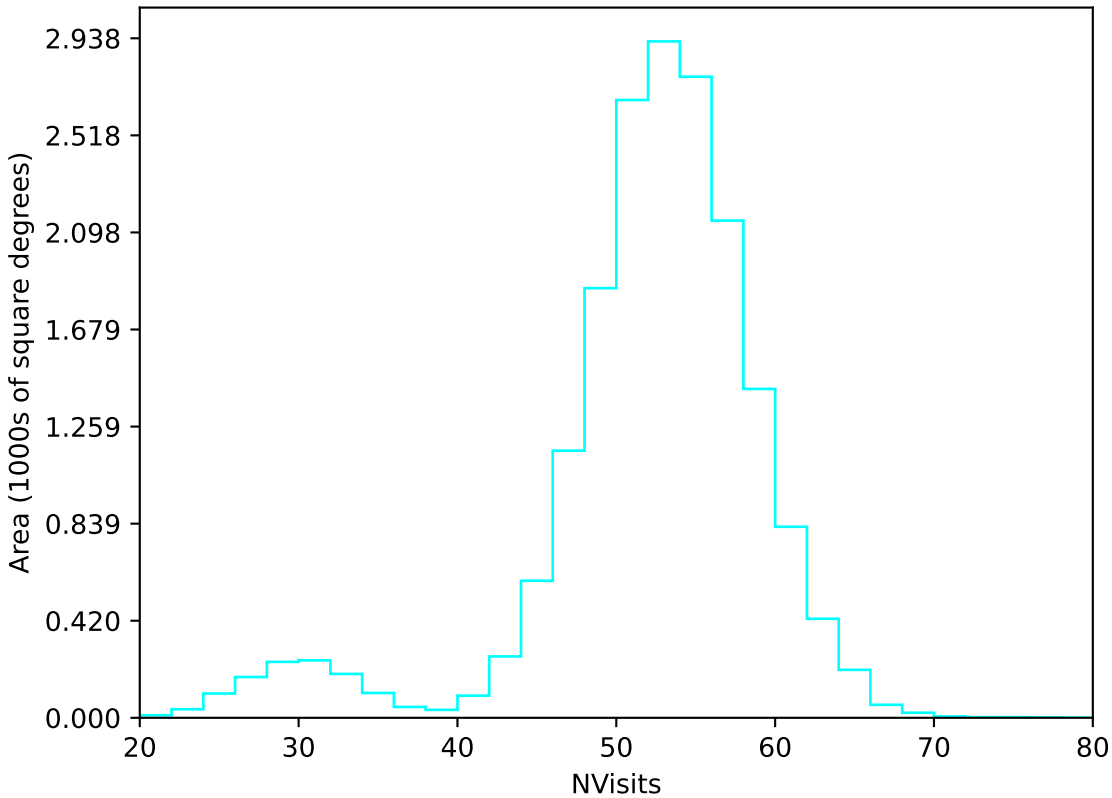
too_elab_heavy_r32_d2_gz_v3.4_10yrs WFD u band: NVisits
