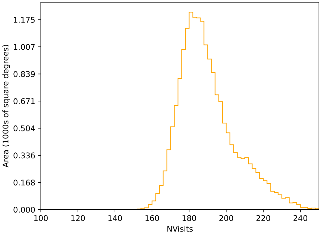
too_elab_heavy_r32_d2_gz_v3.4_10yrs WFD r band: NVisits
