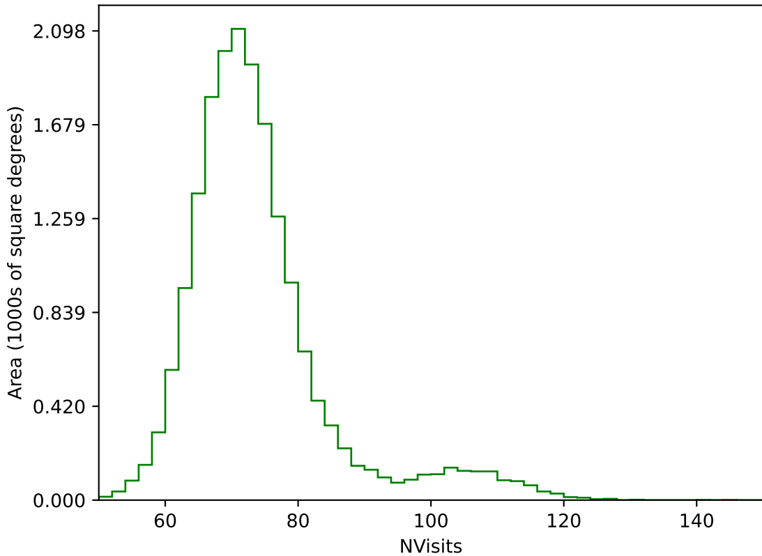
too_elab_heavy_r32_d2_gz_v3.4_10yrs WFD g band: NVisits
