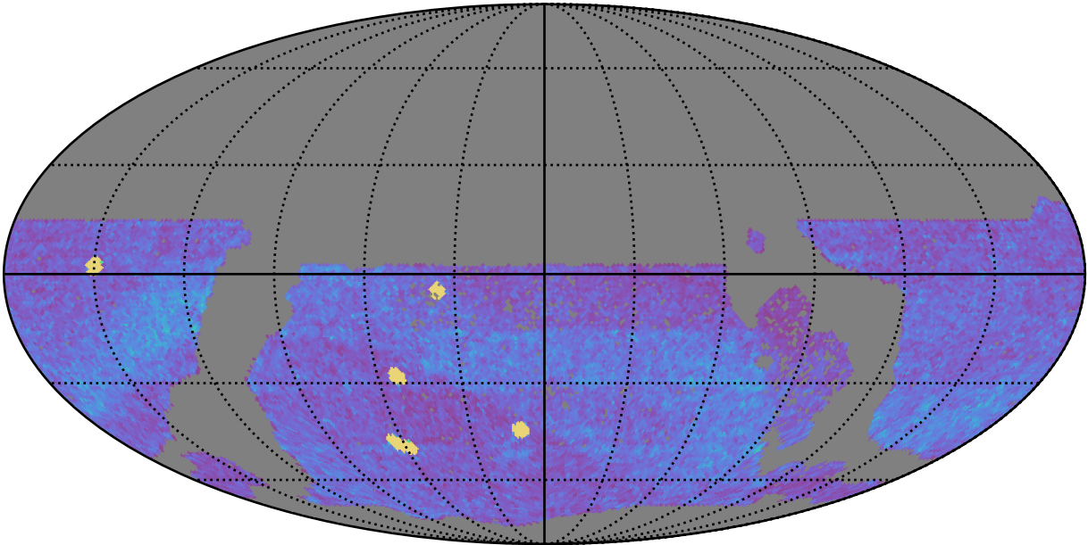
too_elab_heavy_r32_d2_gz_v3.4_10yrs WFD all bands: NVisits
