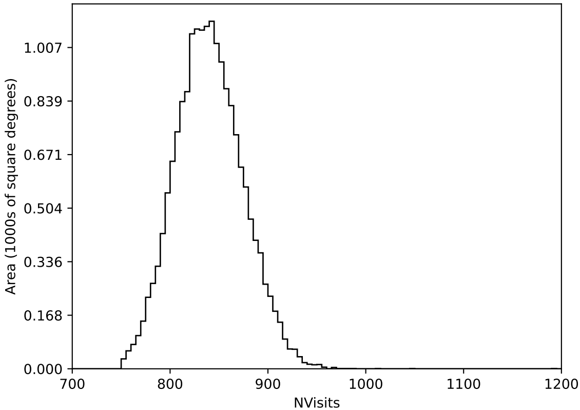
too_elab_heavy_r32_d2_gz_v3.4_10yrs WFD all bands: NVisits
