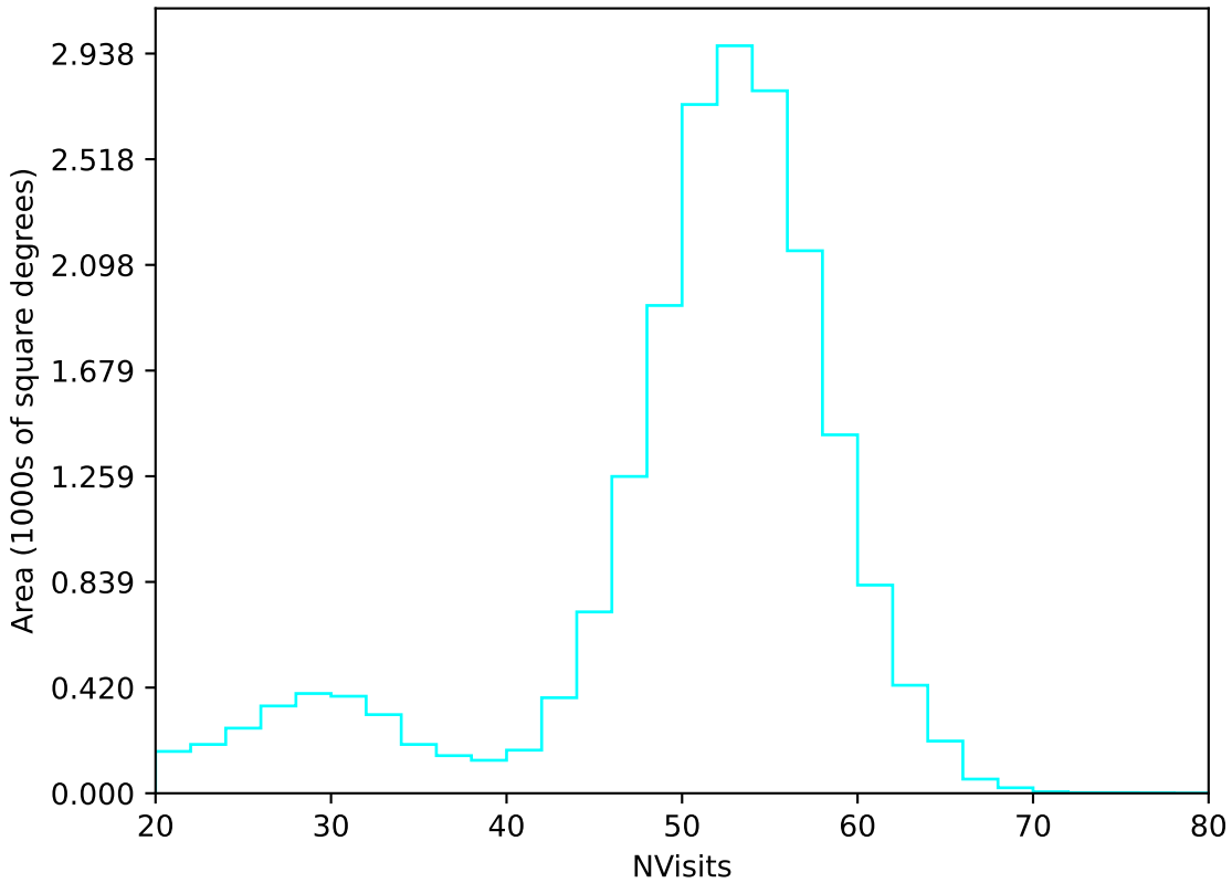
too_elab_heavy_r32_d2_gz_v3.4_10yrs All sky u band: NVisits
