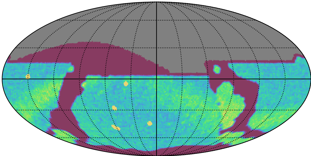
too_elab_heavy_r32_d2_gz_v3.4_10yrs All sky r band: NVisits
