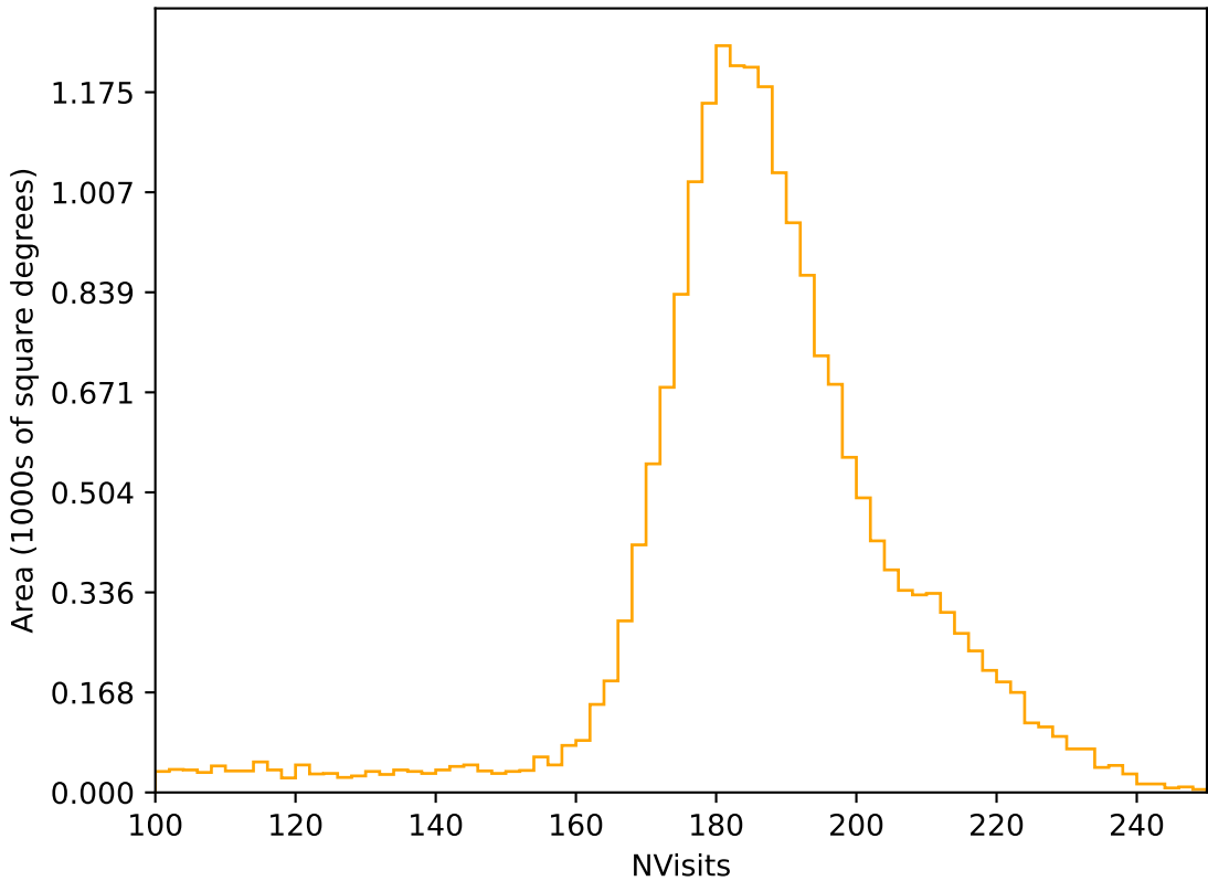
too_elab_heavy_r32_d2_gz_v3.4_10yrs All sky r band: NVisits
