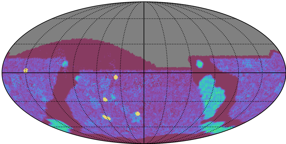
too_elab_heavy_r32_d2_gz_v3.4_10yrs All sky g band: NVisits
