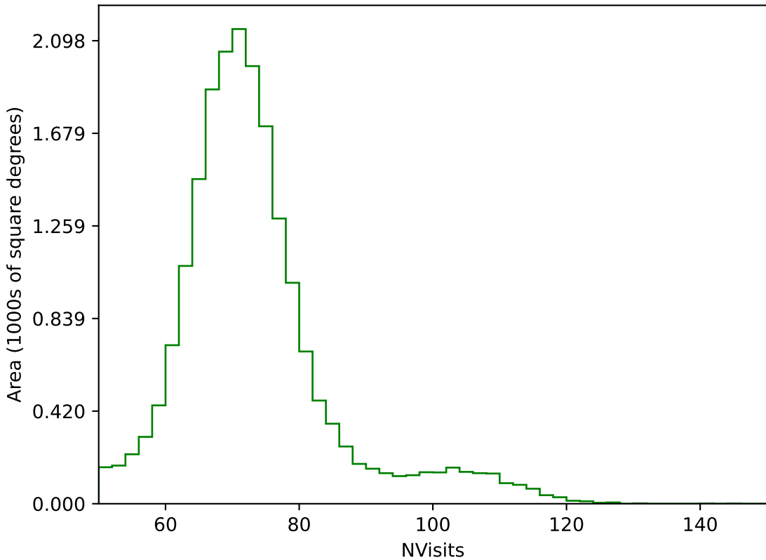
too_elab_heavy_r32_d2_gz_v3.4_10yrs All sky g band: NVisits
