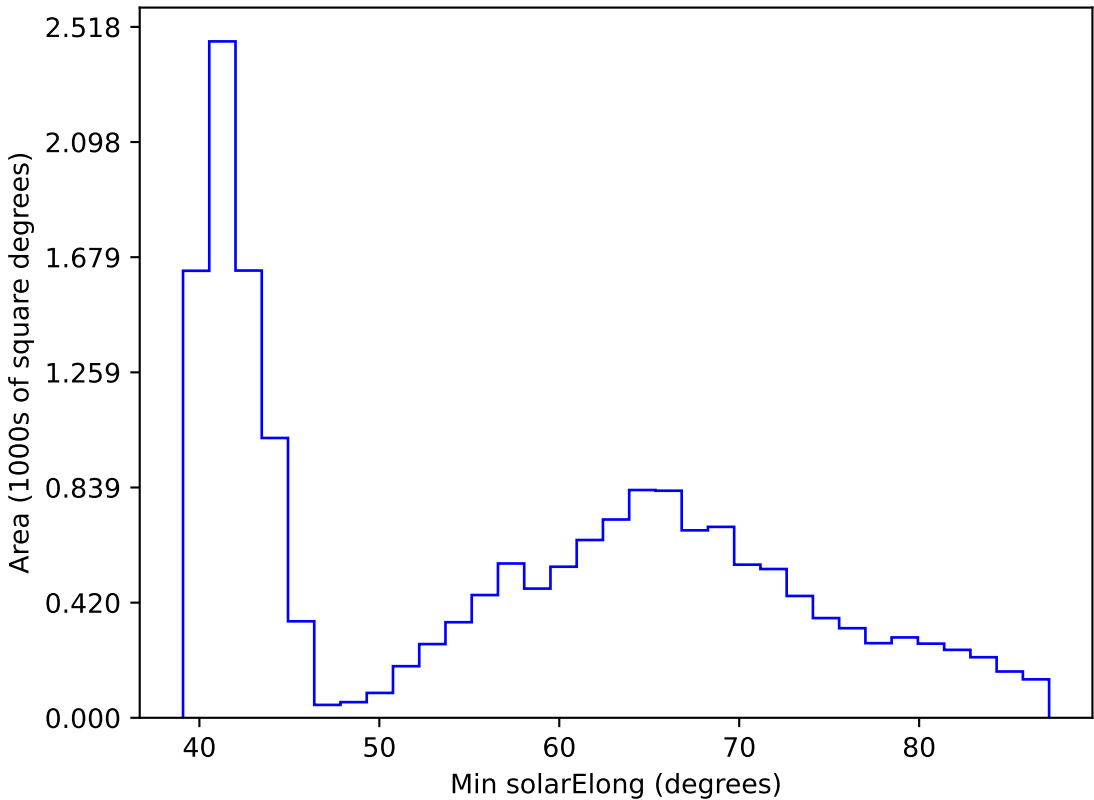
too_elab_heavy_r32_d2_gz_v3.4_10yrs WFD r band: Min solarElong
